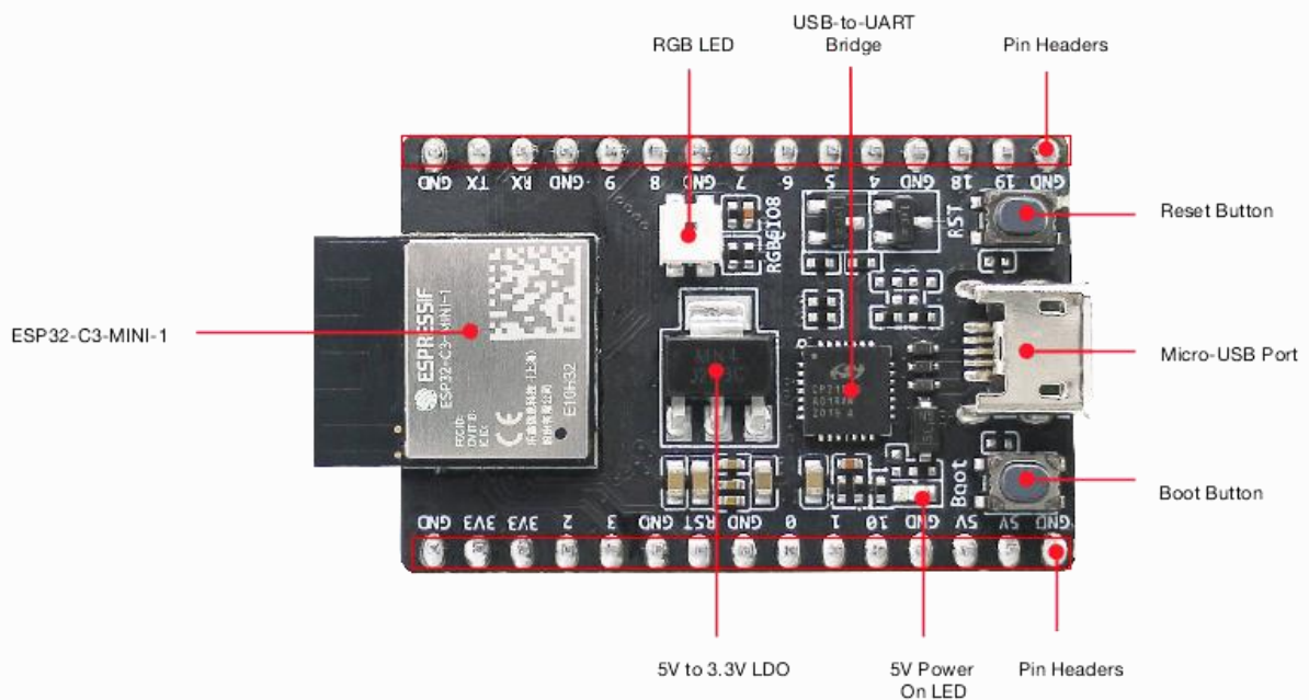
ESP32-C3-DevKitM-1 - front
