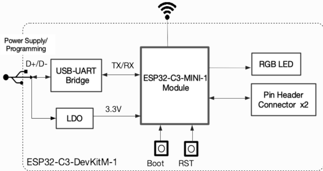
ESP32-C3-DevKitM-1 (click to enlarge)
