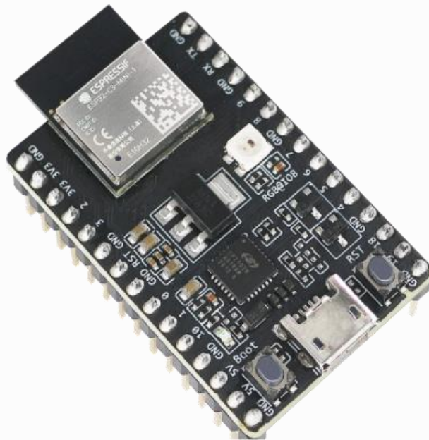
ESP32-C3-DevKitM-1
